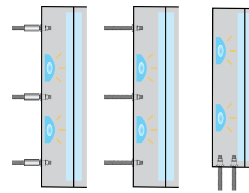
Stud with Spacers
