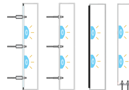
Stud with Spacers
